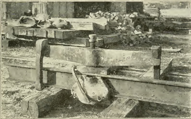
Fig. 229. Apparatus Set for a Cast-Welded Joint
